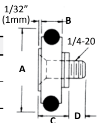
RUBBER TIRE BEARING WITH SCREW STUD STEEL INNER AND OUTER RACE
