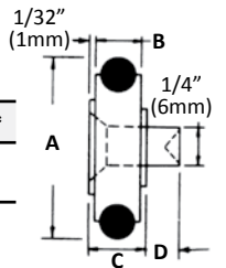
RUBBER TIRE BEARING WITH RIVET STUD STEEL INNER AND OUTER RACE
