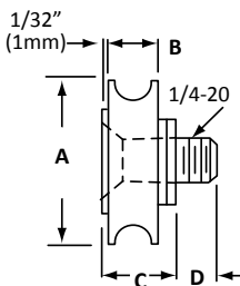
CONCAVE BEARING WITH SCREW STUD STEEL INNER AND OUTER RACE
