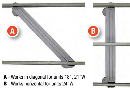
DUNNAGE SUPPORT STAND* QPDS
